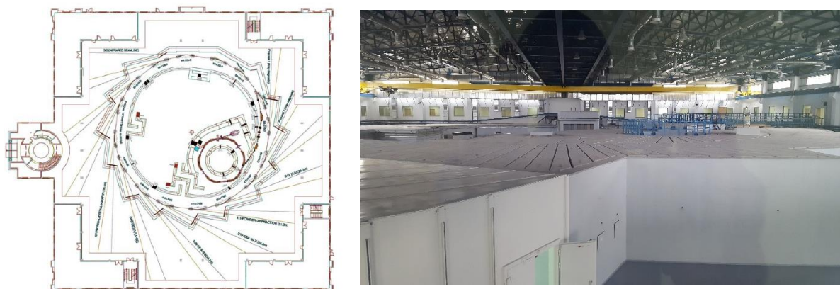
Figure 17: Schematic outline of the SESAME synchrotron facility with storage ring 20 , photo of storage ring, December 2018.
